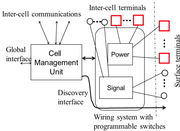
Fig. 19. Functional representation of unit cell. The unit cell transfer information with the cell management unit. The unit cell contains three grids: (i) a mechanical mounting grid (the coarsest grid), (ii) a power terminal grid, and (iii) a signal grid.
