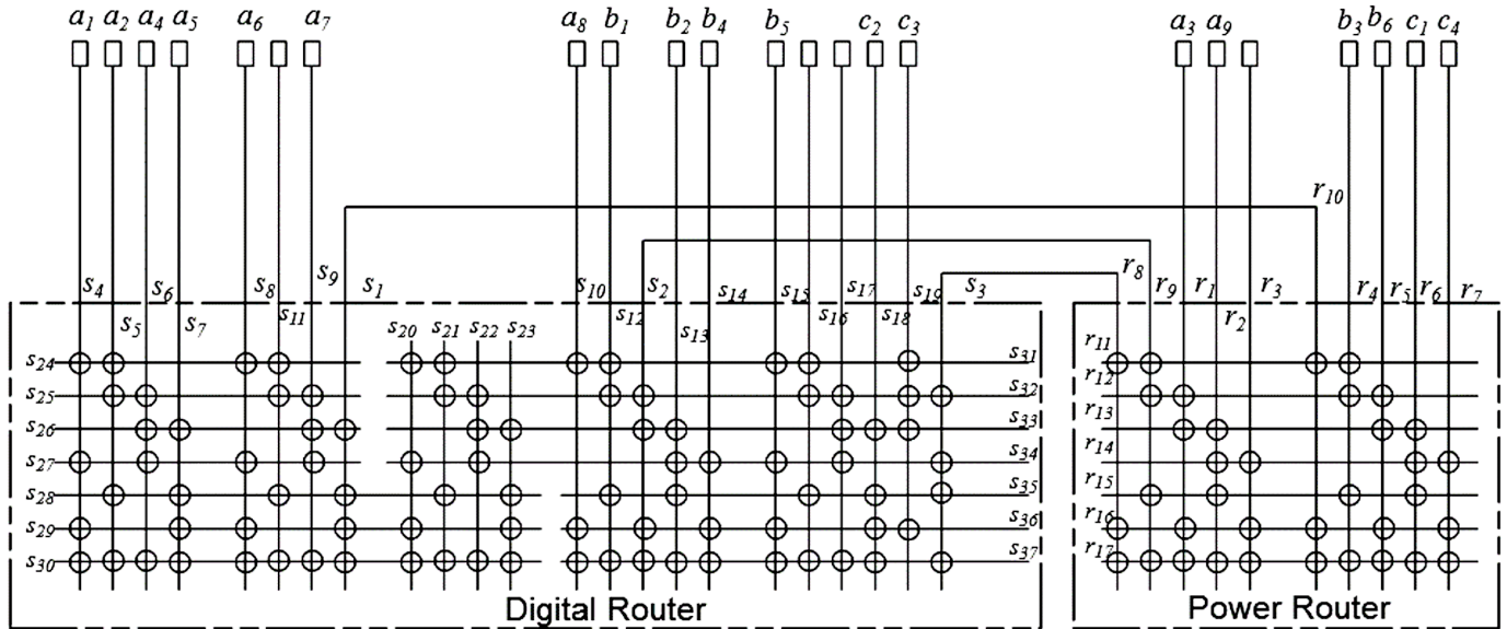
Fig. 6. Programmable resource model. We show an example with two routers, one digital and one power, and a set of external terminals and pinouts. The challenge is to connect different set of terminals using the two routers.
