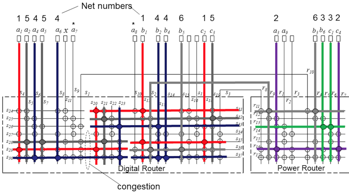
Fig. 7. Sample implementation solution for multi-domain netlist. Using the programmable resource model example from Fig. 6, different terminals are connected using the two routers and their terminals.
