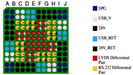
Fig. 16. Pin conventions for distributed contact arrays for prospective use in PnPSat [64].
