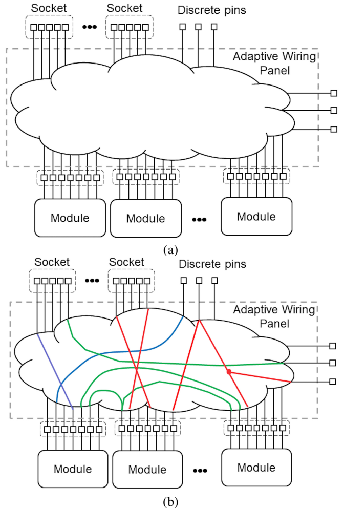
Fig. 1. Programmable wiring manifold. (a) Abstraction. (b) Depicting programmable interconnections.
