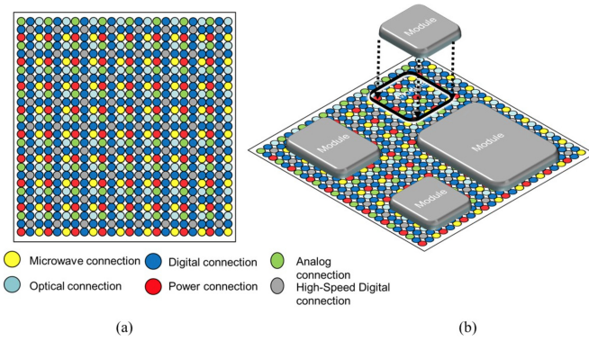
Fig. 8. Adaptive wiring panel (monolithic). (a) Panel depicting a distribution of multi-domain contact points. (b) Depiction of modules placed onto the panel.
