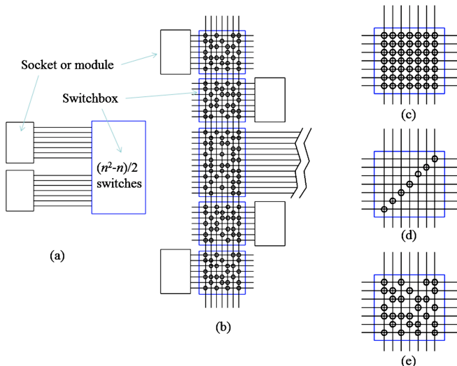
Fig. 10. Elementary fabric concepts. (a) Brute force routing. (b) Segmented hierarchical fabric. (c) Fully populated switchbox. (d) Linear population. (e) Heuristically-determined population.
