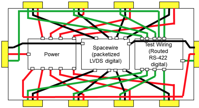
Fig. 15. Simple, multi-domain panel design used in space plug-and-play architecture (SPA) research. In this example, each panel contains a number of ports. Each port contained connections to three limited domains: (i) power (only 28VDC), (ii) a Spacewire [56] packet routing link, and (iii) a serial testing interface, which allowed system-wide injection/query operations in a manner analogous to a JTAG [47] interface.
