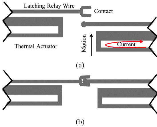
Fig. 12. Bistable MEMS switch design with two lateral thermal switches. (a) Open (b) Closed.
