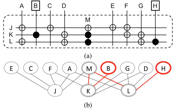
Fig. 4. Very simple programmable panel. (a) Routing resource model of wires and switches. (b) Equivalent graph-theoretic formulation.
