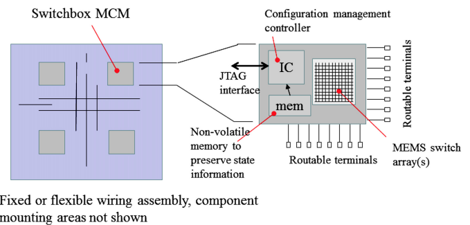
Fig. 11. Multichip module implementation of MEMS-based FPID. This module contains one or more MEMS switch crosspoint arrays and a controller sidecar ASIC.
