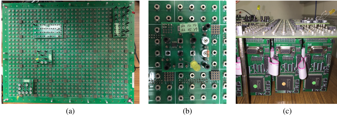
Fig. 20. Images of the final AWP prototype [65]. (a) AWP with some modules placed on top. (b) A single module. (c) Side view showing the circuitry, the panel and the modules on top.
