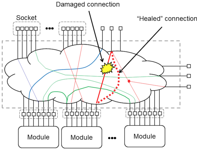
Fig. 3. Repairing faulty connections in adaptive wiring system through circumlocution of damage.
