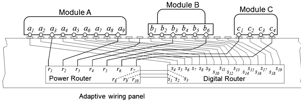
Fig. 5. Second adaptive wiring panel study example. In this case, only programmable connections are shown (i.e. all panel termini connect to active routers). On the other hand, the adaptive wiring panel can also contain a certain fraction of fixed connections.
