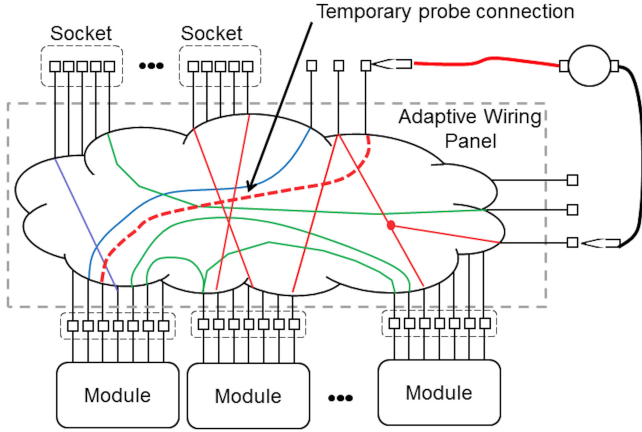
Fig. 2. Temporary connections in an adaptive wiring panel.
