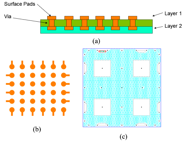
Fig. 13. The “liquid manifold” packaging concepts. (a) Component level land grid array (LGA). (b) Panel LGA pattern. (c) Panel structure design with mounting zones for modules.
