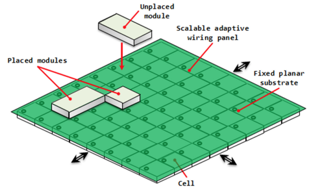
Fig. 17. Adaptive Wiring Panel (AWP) concept [65], [66], [18]: (i) cell units (the basic tile building blocks); (ii) cell management units (CMUs); (iii) modules represented components that plug onto tiled arrays; and (iv) some notion of a global system to manage the set of tiles and to netlist the modules.
