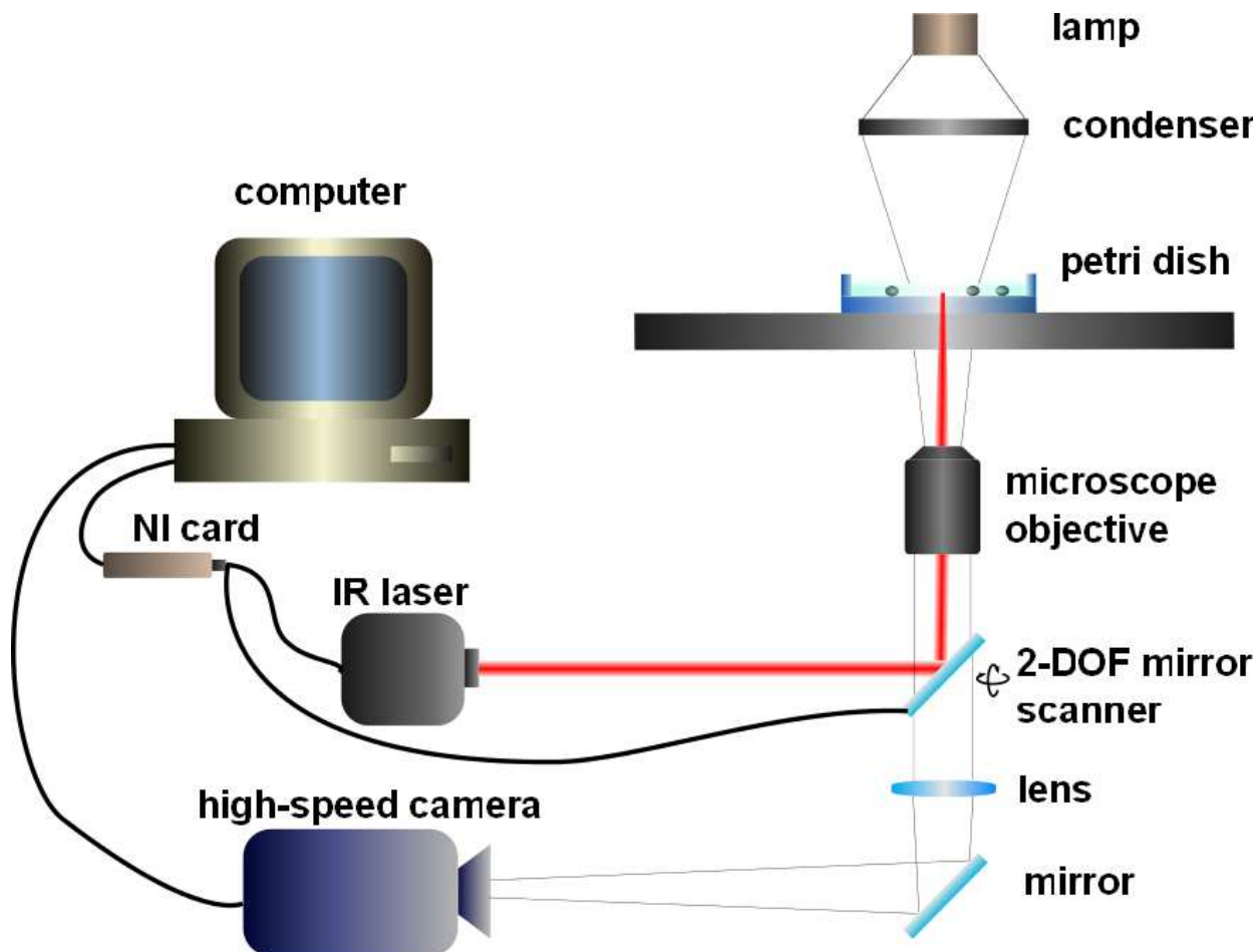
FIG. 1. (Color online) Schematic of the robotic system. A focused IR laser beam is addressed by a mirror scanner into the sample. A high-speed camera monitored and provided bead positions for visual servoing.
