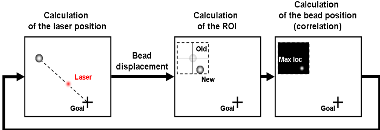
FIG. 4. (Color online) Schematics of the tracking method using image correlation. The laser is shot at a distance d from the bead to handle it, the bead moves towards the laser beam and then the ROI image updates its position in order to not to lose the future bead position. Once the bead position computed, the laser is shot again at the same distance d . This continues until beads reach their target positions.
